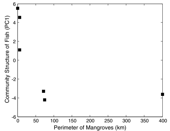
Fig. 2 – Relationship between availability of mangrove nursery habitat and the community structure of coral reef fish on outer Montastraea reefs. Community structure based on the mean biomass of 162 species in each reef system where each system was sampled in at least three locations. The first principal component explained 39% of variation in the data.
