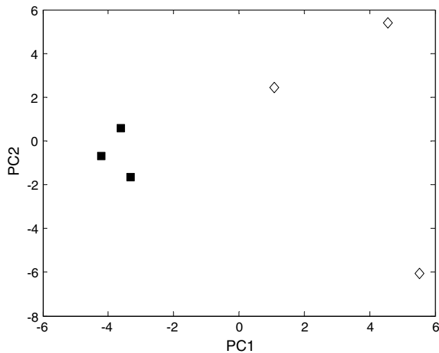
Fig. 1 – Principal Components ordination of the community structure of coral reef fishes in six reef systems throughout Belize and Mexico. Mangrove-rich systems (■) include Turneffe Atoll, Tobacco Range and Curlew Cay. Systems with scarce mangroves (◇) include Banco Chinchorro, Glovers Reef and Lighthouse Reef.
