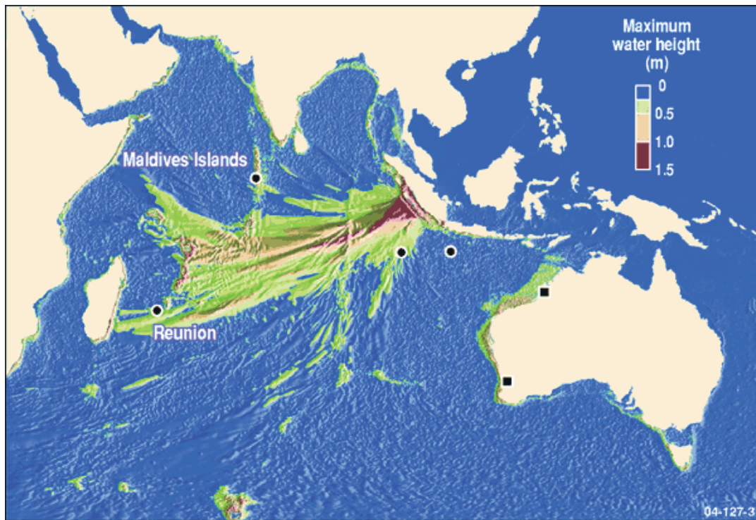
Figure 18. Calculated maximum amplitude of the tsunami caused by the 1833 Sumatra earthquake. Most tsunami energy was directed in a southwesterly direction into the open Indian Ocean (Numerical modelling performed by David Burbidge of Geoscience Australia; http://www.ga.gov.au/ausgeonews/ausgeonews200503/tsunami.jsp )
